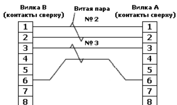
Plug A (contacts on top) Twisted pair Plug B (contacts on top)
