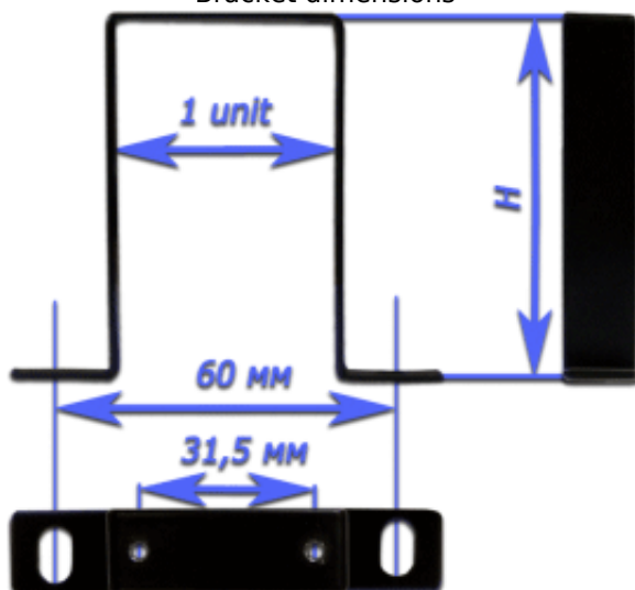
Bracket dimensions
