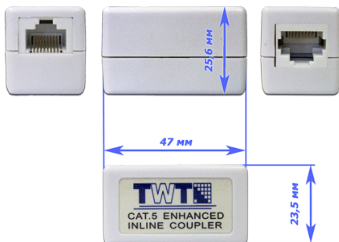
Coupler Dimensions
