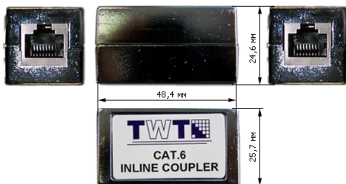
Coupler dimensions
