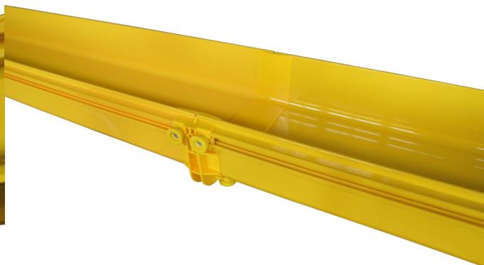
Joining of two 240 mm wide straight sections, top view
