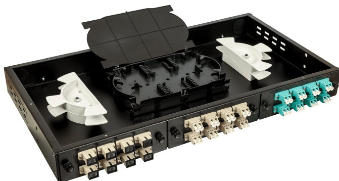
Splice tray with removed cover
